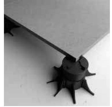
PAVIMENTO ELEVADO RAISED FLOORING SYSTEM POSE SURÉLEVÉE
