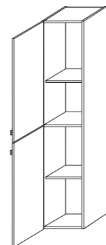
E 35.07 L,D Visoka omara I,D Visoki ormar I,D Tall cabinet I,R Hochschrank I,R • 35/160/35 149,59 PT *
