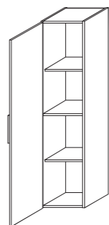
D 35.07 L,D Visoka omara L,D Visoki ormar L,D Tall cabinet L,R Hochschrank L,R • 35/130/30 113,22 PT *
